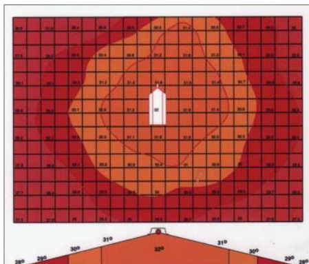
*Fig 2: Temp. difference is the temperature difference from the center of the brooding area to the end of the coverage area.
